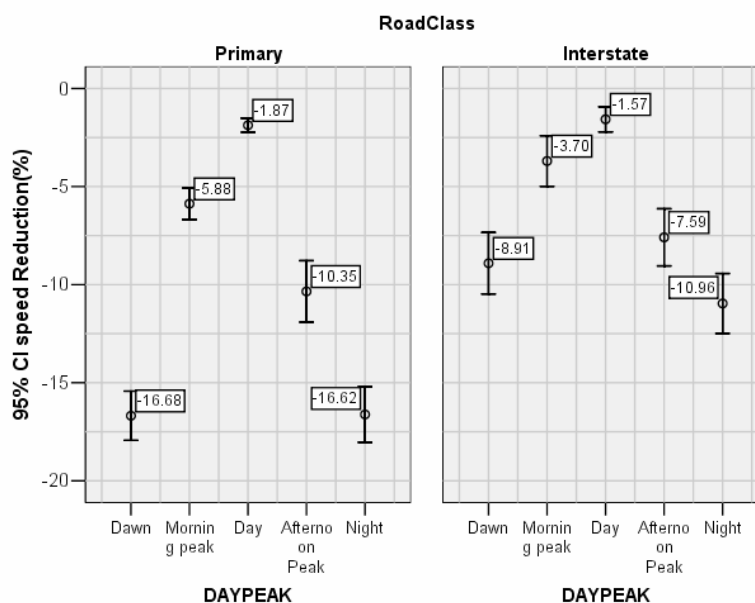
Figure VI-7. Speed deduction for highways with speed limit 65 mph and AADT 1-5K
